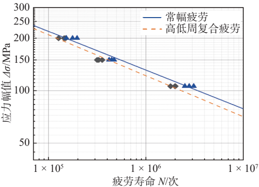
图 4 Type-1 类型接头高低周复合疲劳 S-N 曲线与常幅疲劳 S-N 曲线 Fig. 4 S-N curves of combined high and low cycle fatigue tests and constant amplitude fatigue tests of Type-1 welded joints
