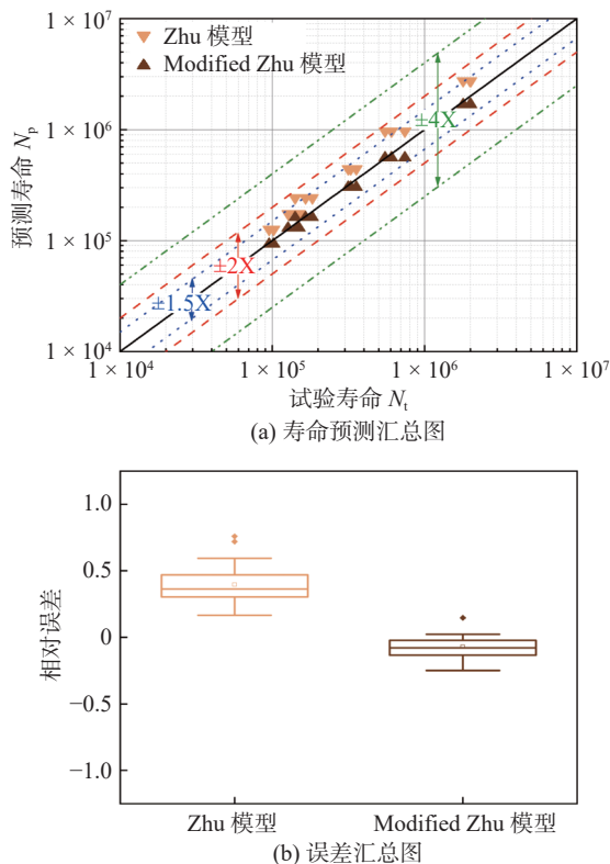
图 11 修改前后 Zhu 模型寿命预测图和误差箱线图 Fig. 11 Life prediction and error of Zhu model. (a) life prediction of Zhu model; (b) error of Zhu model
